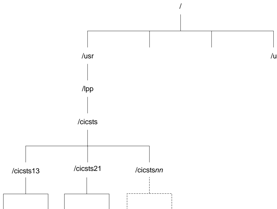
Figure 2. The HFS directory structure for CICS java and IIOF files
