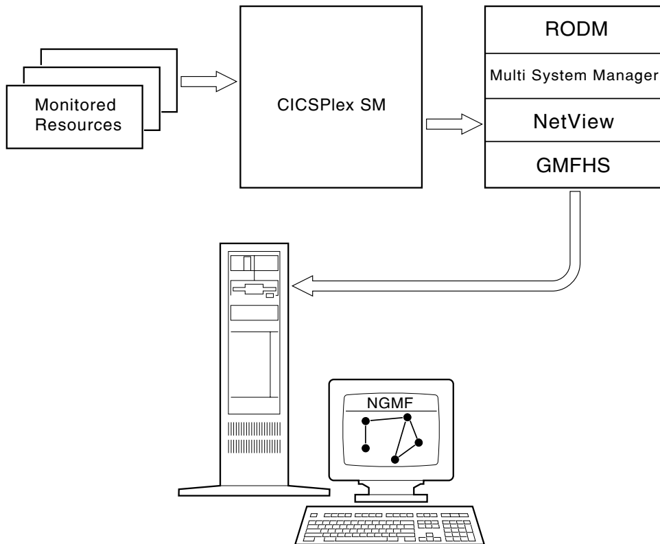
Figure 60. Components of the CICSPlex SM RODM interface
