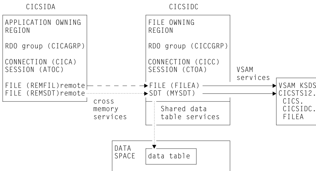
Figure 37. CICS environment for example verification of shared data tables
