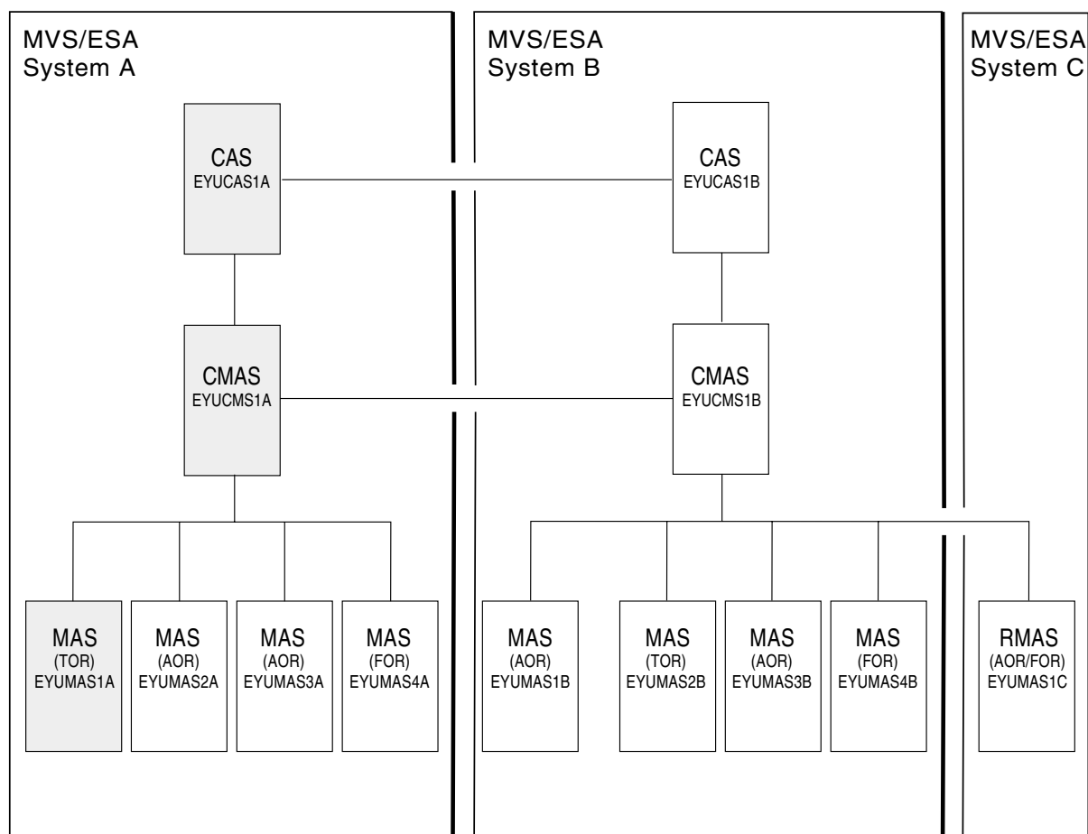
Figure 62. Starter Set components for IVP1. Shaded components—EYUCAS1A, EYUCMS1A, and EYUMAS1A—are used during IVP1
