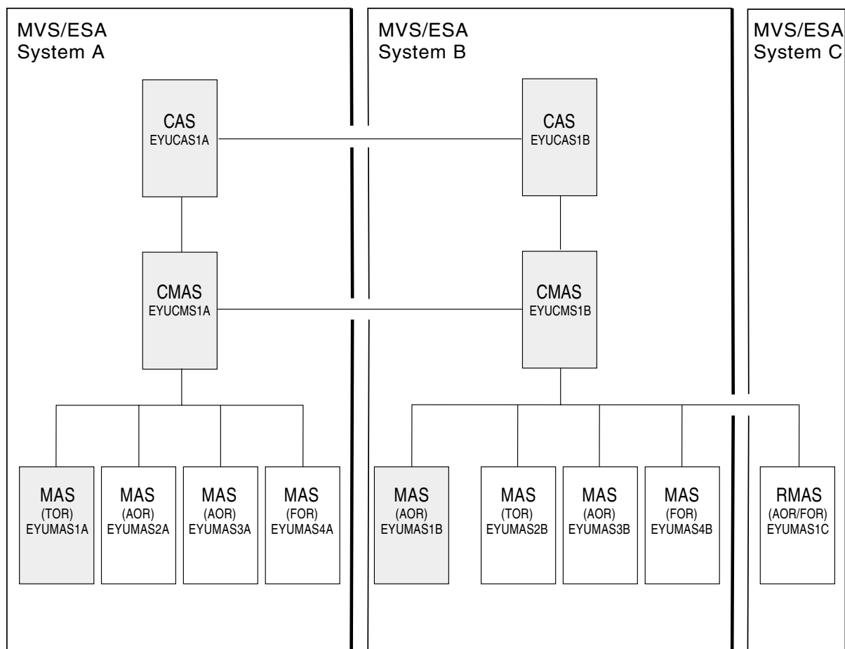
Figure 63. Starter Set components for IVP2. Shaded components—EYUCAS1A, EYUCAS1B, EYUCMS1A, EYUCMS1B, EYUMAS1A, and EYUMAS1B—are used during IVP2.
